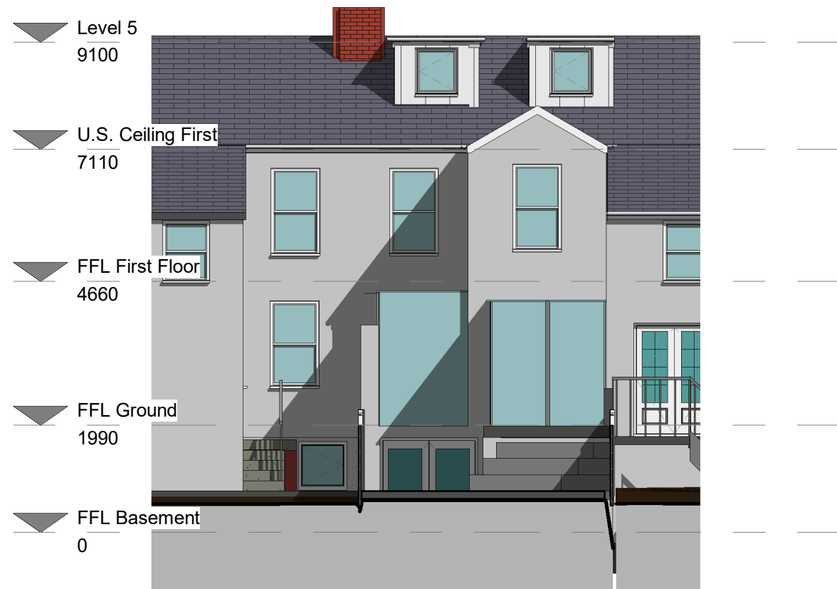
4 South Proposed Spring 1 : 100
